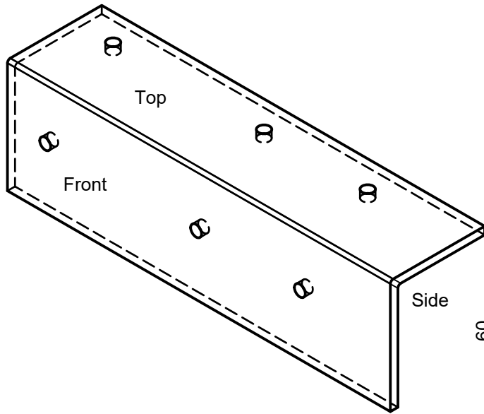
L_Bracket_Leg_left-version_Drawing
